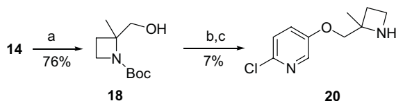
Scheme 4. Reagents: (a) \text{LiBH}_4 , MeOH, \text{Et}_2\text{O} ; (b) 2-chloro-5-hydroxypyridine, \text{Ph}_3\text{P} , DEAD, THF; (c) TosOH, EtOH.
