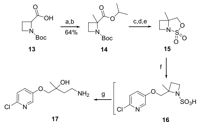
Scheme 3. Reagents and conditions: (a) i -PrOH, EDC, DMAP, CH 2 Cl 2 ; (b) LDA, THF, then MeI; (c) MeSO 3 H, CH 2 Cl 2 ; (d) LiAlH 4 , THF; (e) SO 2 Cl 2 , CH 2 Cl 2 , –78 °C; (f) 2-chloro-5-hydroxypyridine, NaH, DMF; (g) 20% H 2 SO 4 , 80 °C.
