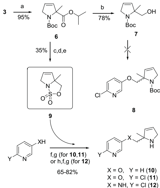
Scheme 2. Reagents and conditions: (a) Li, NH 3 , NH(CH 2 CH 2 OCH 3 ) 2 , THF, –78 °C, then MeI; (b) LiBH 4 , MeOH, Et 2 O; (c) MeSO 3 H, CH 2 Cl 2 ; (d) LiAlH 4 , THF; (e) SO 2 Cl 2 , CH 2 Cl 2 , –78 °C; (f) 9, NaH, DMF; (g) 20% H 2 SO 4 , 90 °C; (h) Boc 2 O, DMAP, CH 3 CN.
