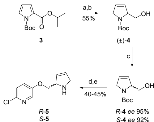
Scheme 1. Reagents and conditions: (a) Na, NH 3 , THF, –78 °C; (b) LiBH 4 , MeOH, Et 2 O; (c) vinylacetate, Pseudomonas fluorescens , t -BuOMe, then (only for S -4) NaOH, H 2 O; (d) 2-chloro-5-hydroxypyridine, Ph 3 P, DEAD, THF; (e) TosOH, EtOH.
